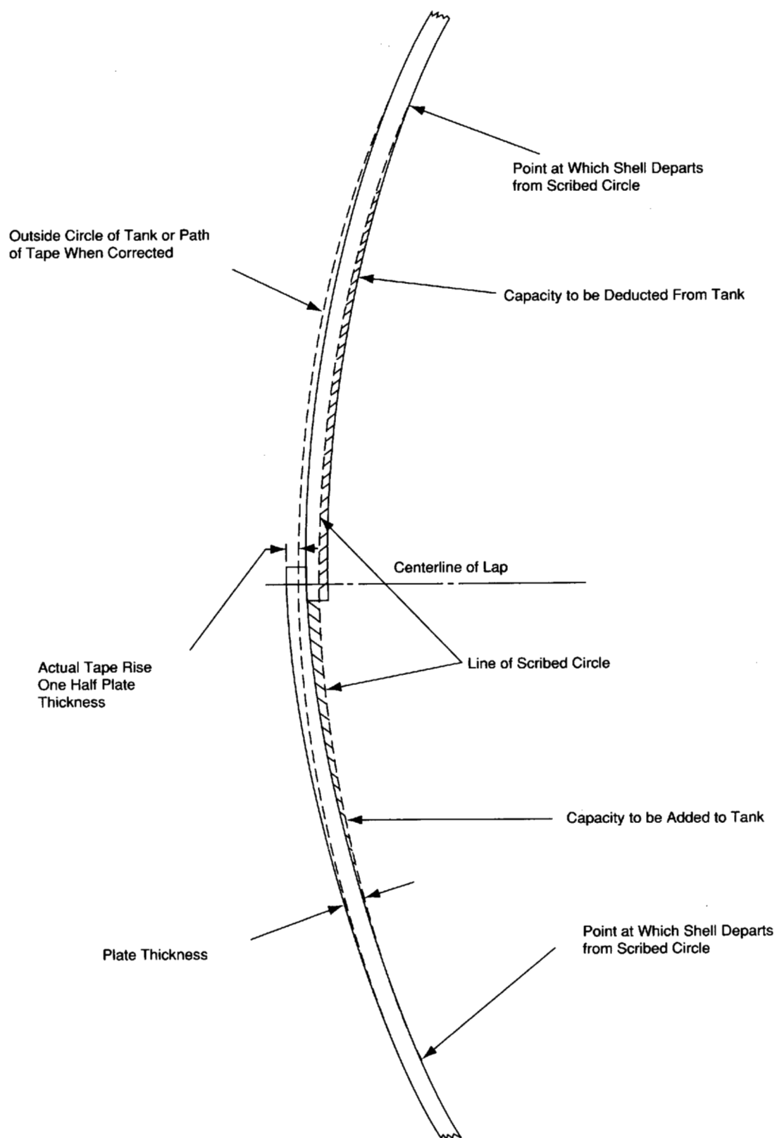
Figure 17—True Circumference Versus Tape Path at Axial Lap Joint Away from Circumferential Joint
