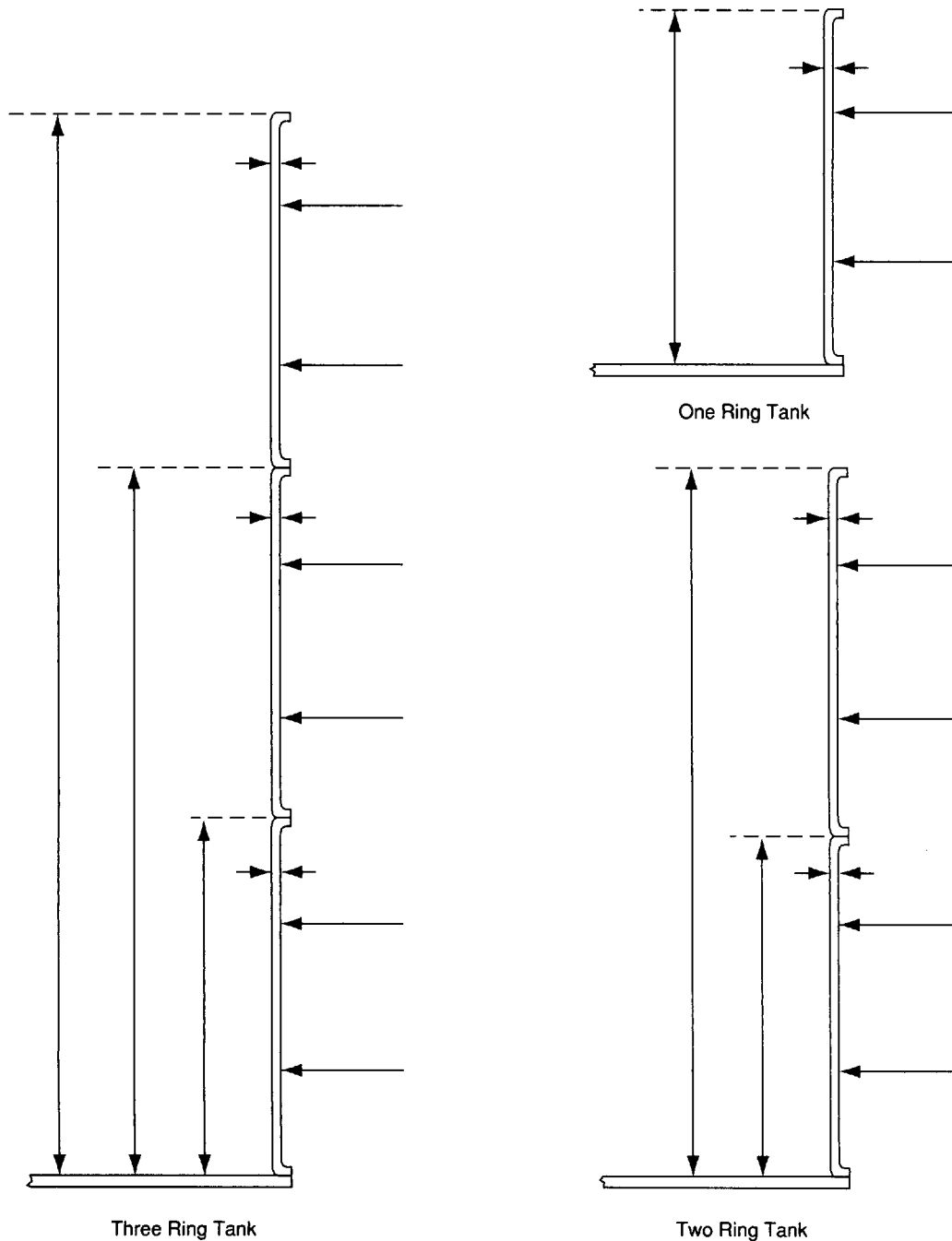
Figure 7—Measurement Locations for Bolted Tanks
