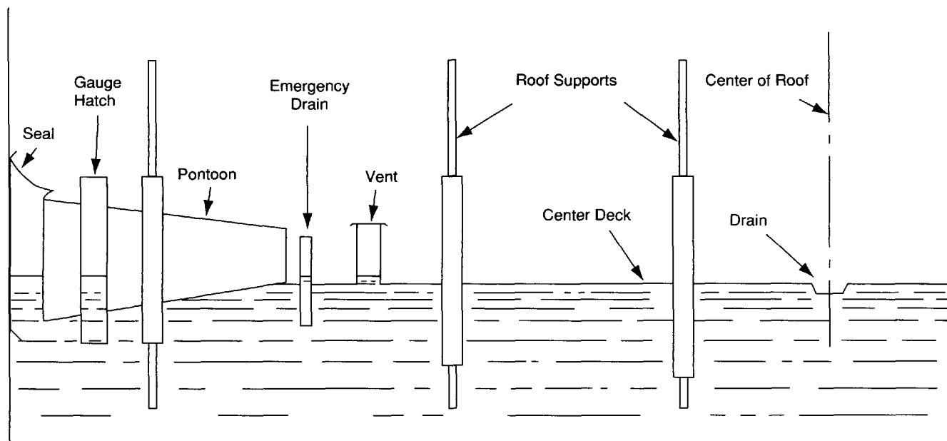
Figure 16—Typical Steel Pontoon Floating Roof with Single Center Deck
